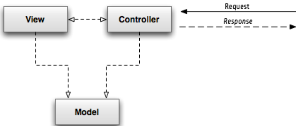
Figure 1.1. Model-View-Controller Pattern
