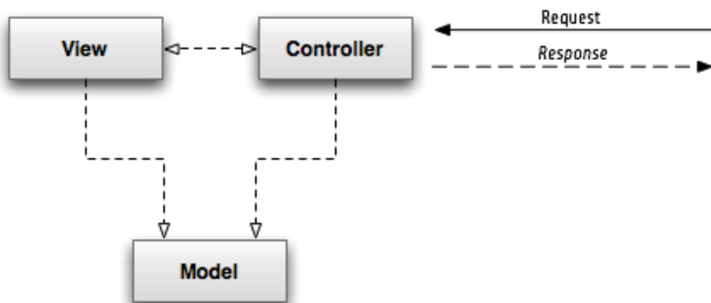
Figure 7.1. Model-View-Controller Pattern
