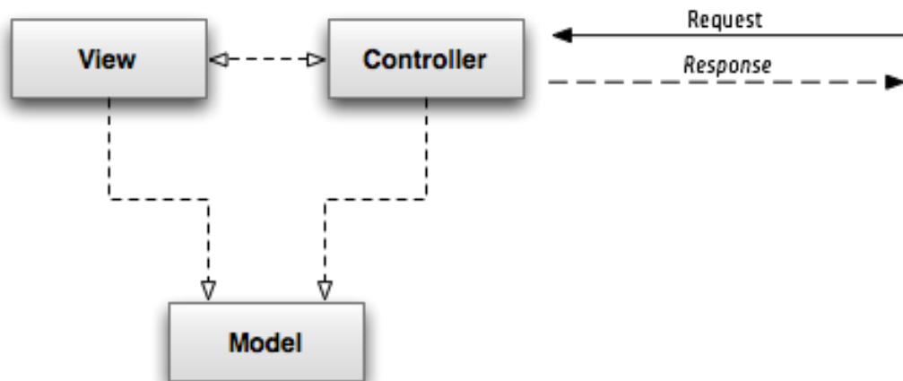
Figure 7.1. Model-View-Controller Pattern
